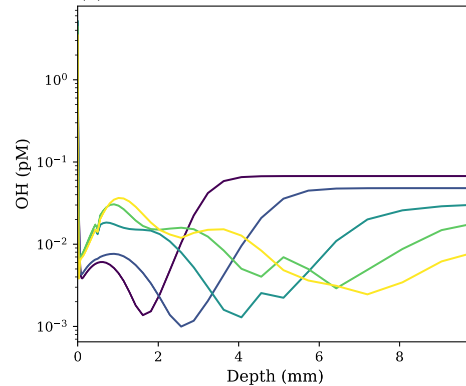
(e) OH
