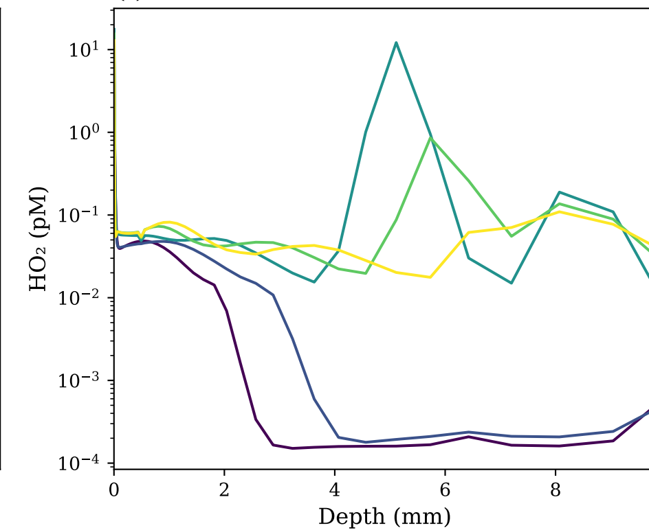
(f) \text{HO}_2
